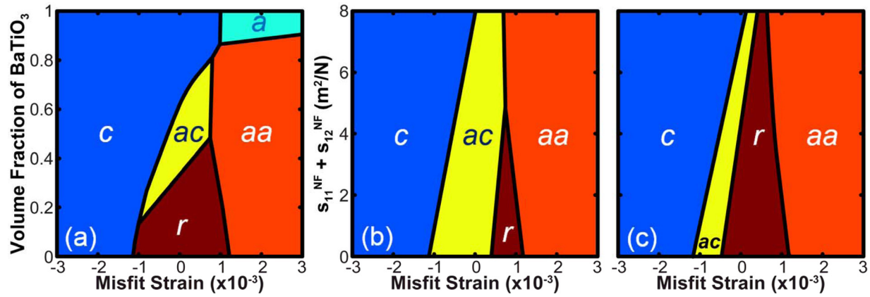
FIG. 2. (a) Volume fraction–misfit strain phase diagram of non-ferroelectric/BaTiO 3 /non-ferroelectric free-standing trilayer heterostructure at T = 25^\circ\text{C} assuming equivalent elastic compliances between the layers ( S_{ij}^F = S_{ij}^{NF} ). Elastic compliance–misfit strain phase diagram of non-ferroelectric/BaTiO 3 /non-ferroelectric free-standing trilayer heterostructure for (b) S_{11}^{NF} - S_{12}^{NF} = 12.25 \times 10^{-12} \text{ m}^2/\text{N} and (c) S_{11}^{NF} - S_{12}^{NF} = 5.38 \times 10^{-12} \text{ m}^2/\text{N} with equal layer thickness ( \phi_F = 0.5 ) at T = 25^\circ\text{C} .
