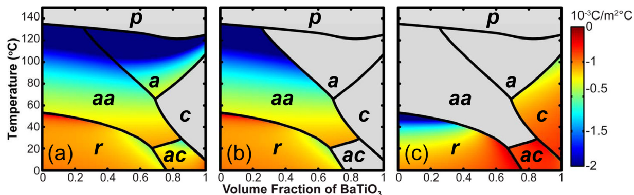
FIG. 4. Pyroelectric coefficients as functions of temperature and volume fraction along (a) [100], (b) [010], and (c) [001] of the \text{NdScO}_3/\text{BaTiO}_3/\text{NdScO}_3 trilayer heterostructures.
